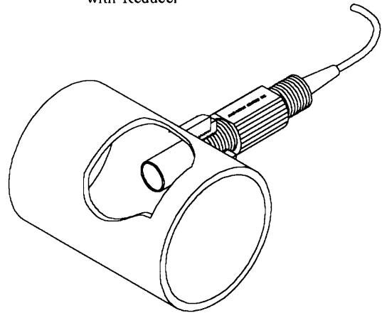
View 2 Pipeline Installation with Reducer
